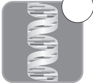
DNA
